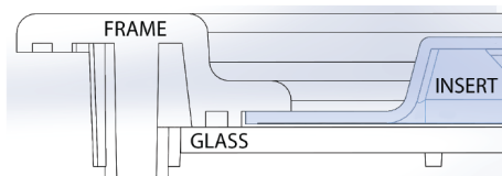
• Snap-in-insert from front of frame with glass sealed to frame
