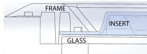
• Lay-in-insert from front of frame with insert sealed to frame
